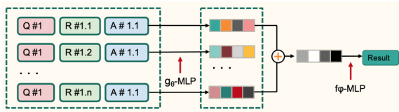
Figure 4: SFRN schematic: encoder (Left); fusion function (Middle); classifier (Right)
