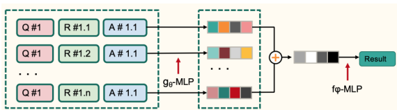
Figure 7: The g_{\theta} MLP function computes the relation vector for each [Q,R,A] triple. A set of relation vectors is combined (+) using SFT. The f_{\phi} MLP function is the assessment classifier.
